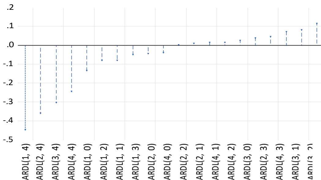
Figure 2. Model Selection over Akaike Information Criteria.
