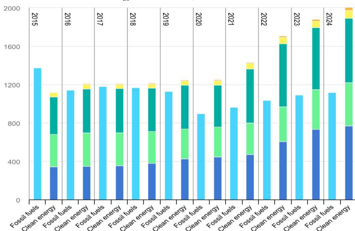
Global investment in clean energy and fossil fuels, 2015-2024 5
