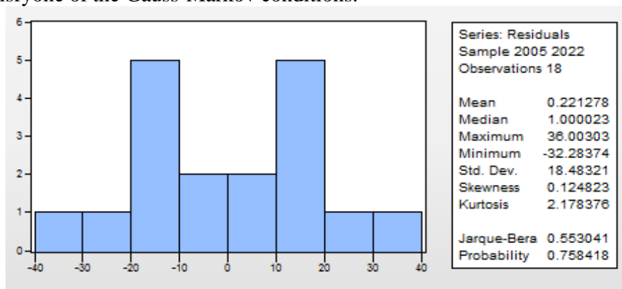
Figure 1. Test of normality of residuals
