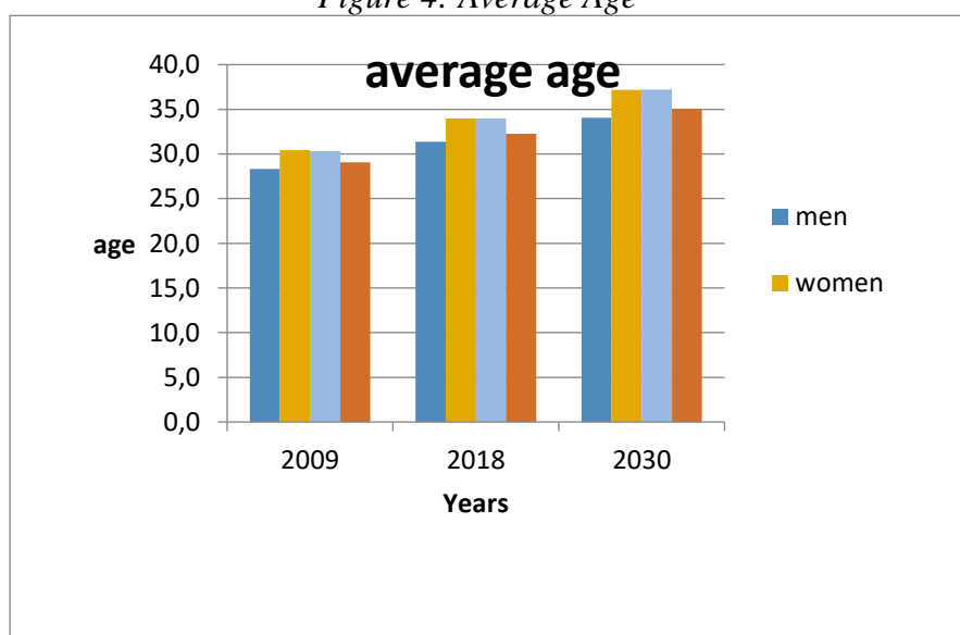
Figure 4: Average Age
