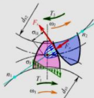
Fig. 1. Forces that act in the engagement of toothed wheels' teeth
