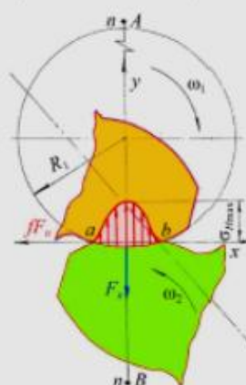
Fig. 2. Estimation scheme to build the refined method for calculating toothed gears in terms of contact strength
