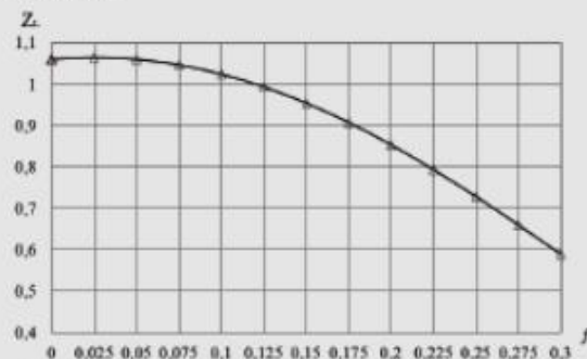
Fig. 3. Dependence graph of a lubricant influence coefficient on friction coefficient
