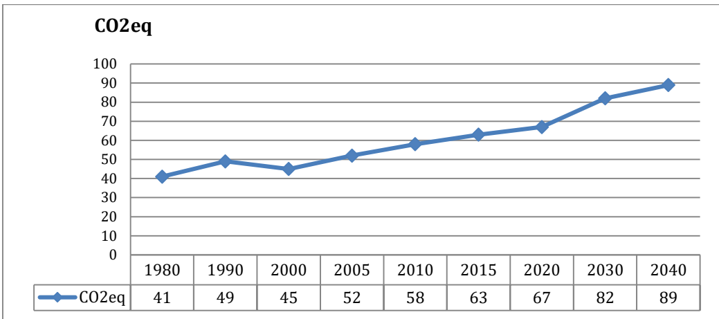
Graph2. Greenhouse gas emissions and target reduction levels to keep global warming within
